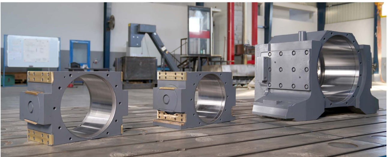
Chocks for Flat Mill
