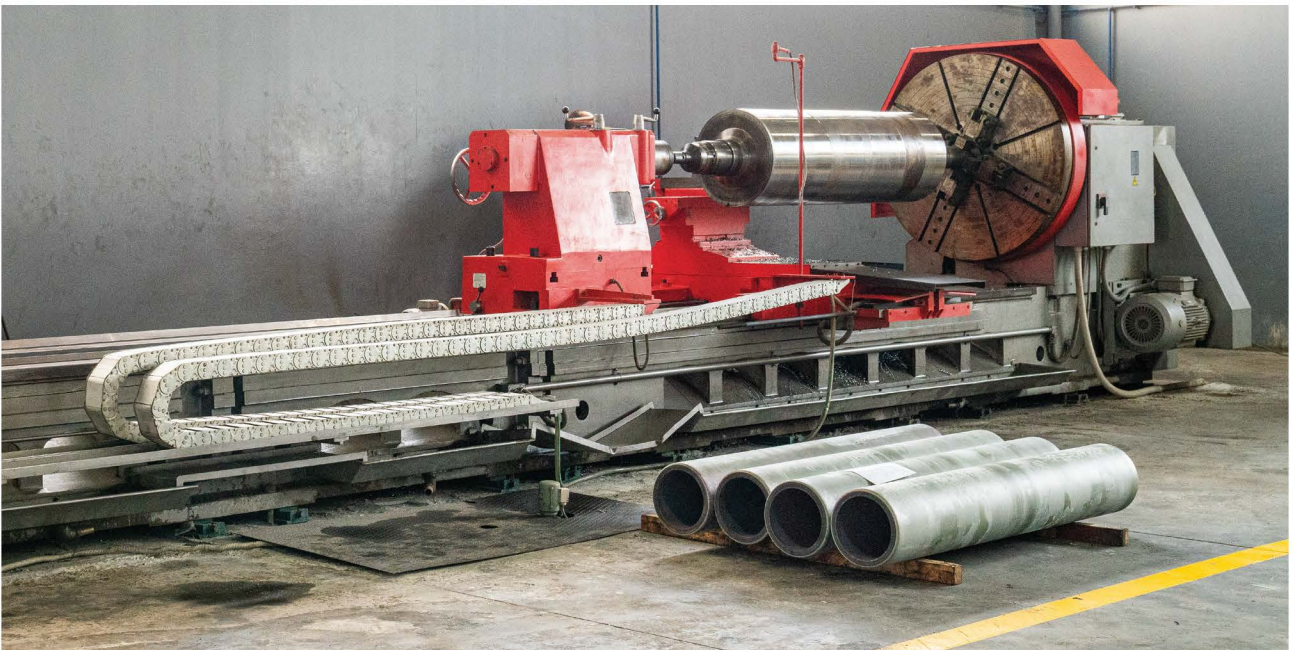
Heavy Duty Turning / 10 Ton Capacity
