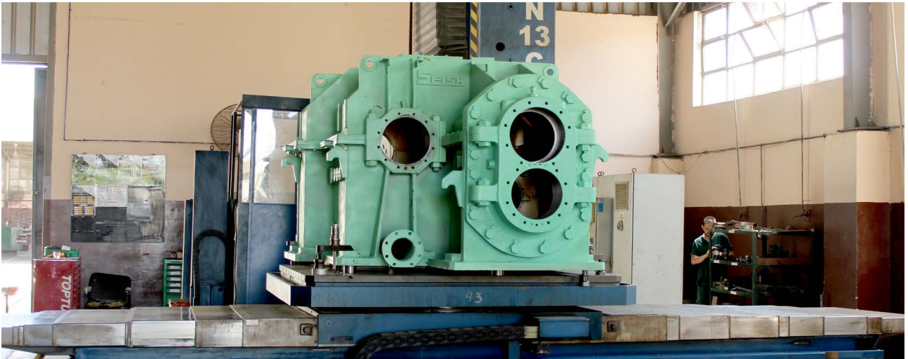
GearBox Housing
